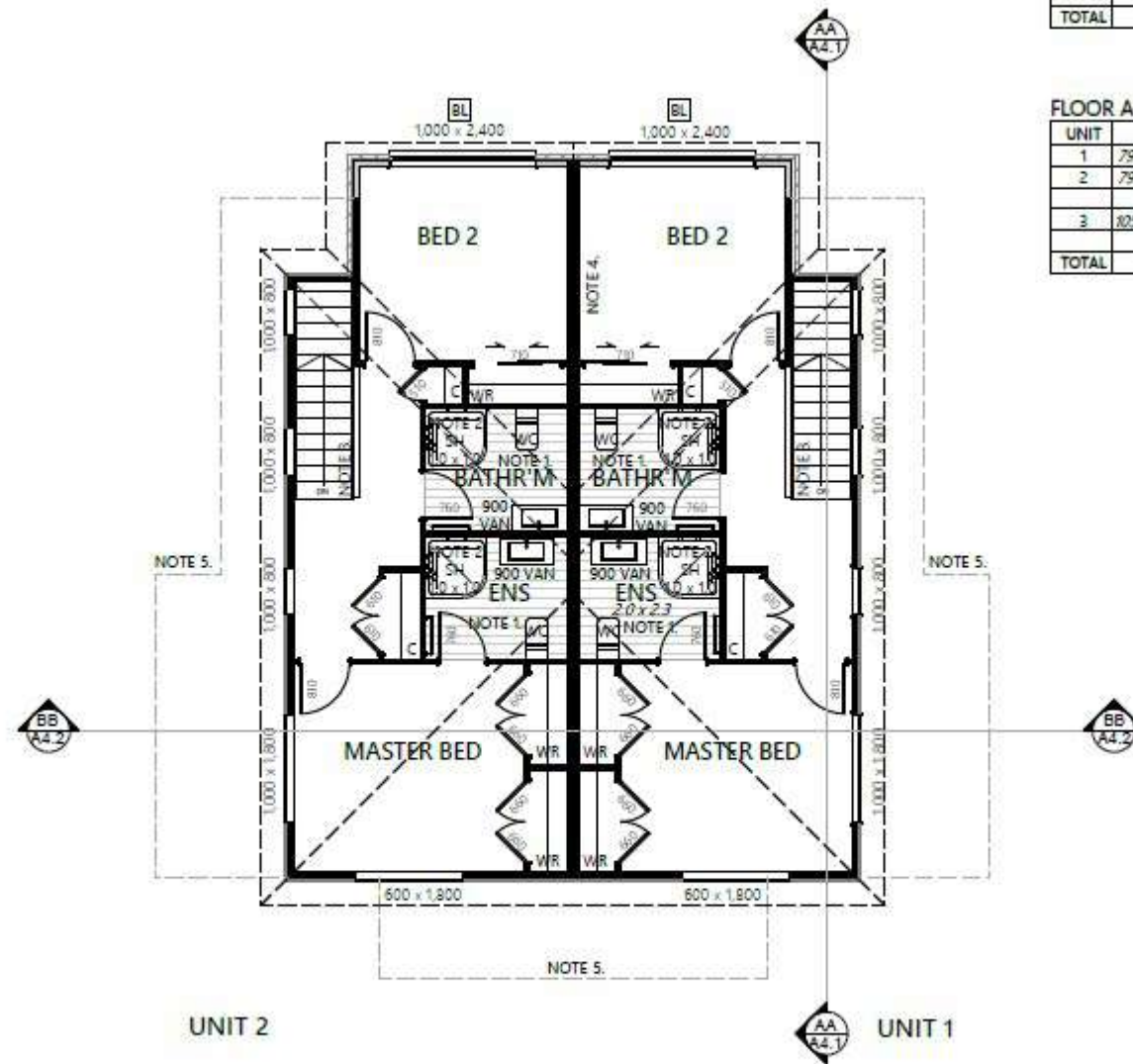
1 FIRST FLOOR PLAN STUD HEIGHT TO BE 2.455m
